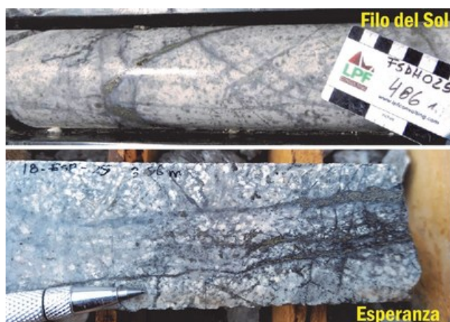
Figure 2: White bleaching (sericite) and D vein (pyrite with white haloes) stockwork development, potential evidence of a strongly telescoped system where a deep porphyry drives a sericite overprint onto a shallower zone. (CNW Group/Libero Copper & Gold Corporation.)
