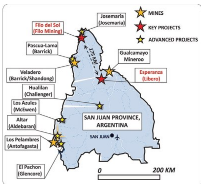
Figure 1: Distribution of major exploration and mining projects in San Juan Province, Argentina (CNW Group/Libero Copper & Gold Corporation.)
