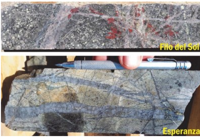
Figure 3: Dense quartz-vein stockwork zones coupled with brown biotite alteration. Alteration styles in porphyry deposits that are often associated with robust Cu-Au mineralization. (CNW Group/Libero Copper & Gold Corporation.)
